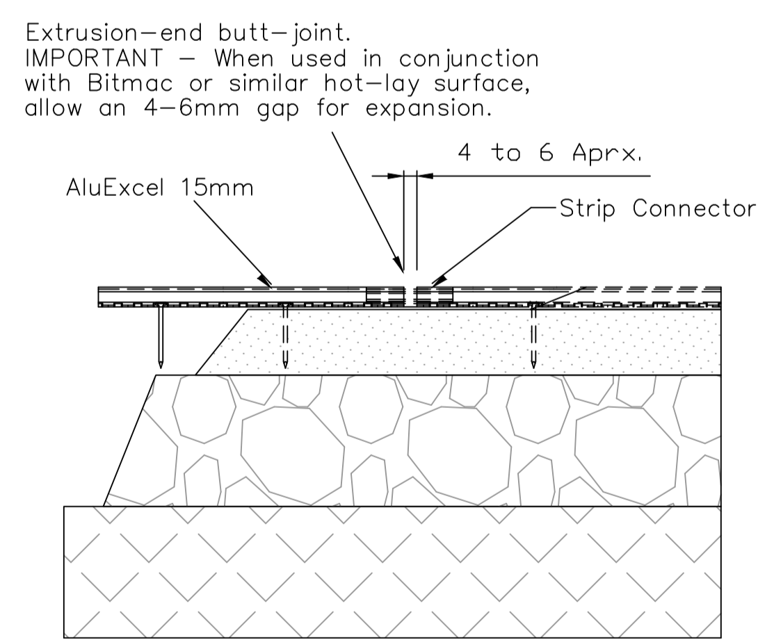
JOINER DETAIL SCALE 1:4
