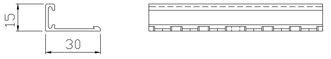
PROFILE DETAIL SCALE 1:1
