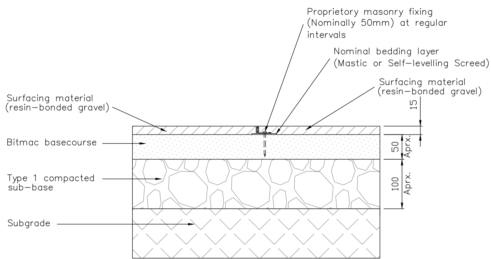
SECTION SCALE 1:4
