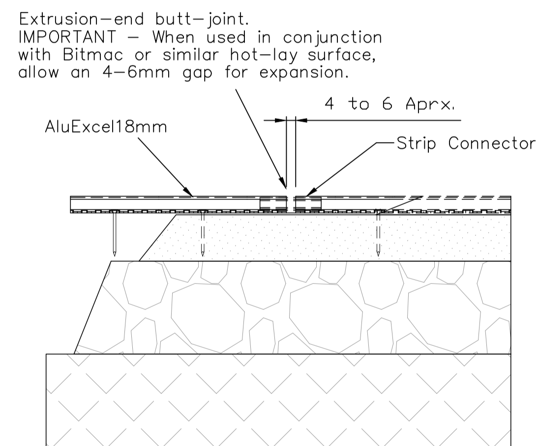
JOINER DETAIL SCALE 1:4
