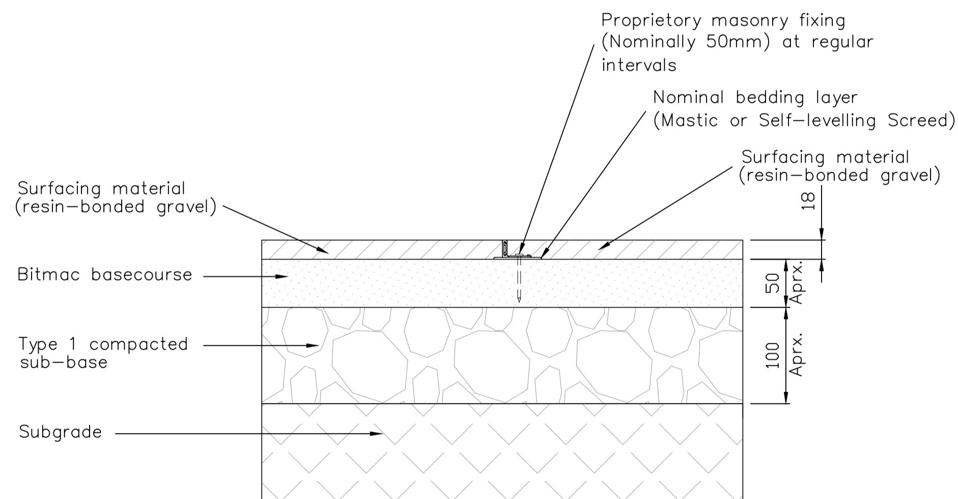
SECTION SCALE 1:4
