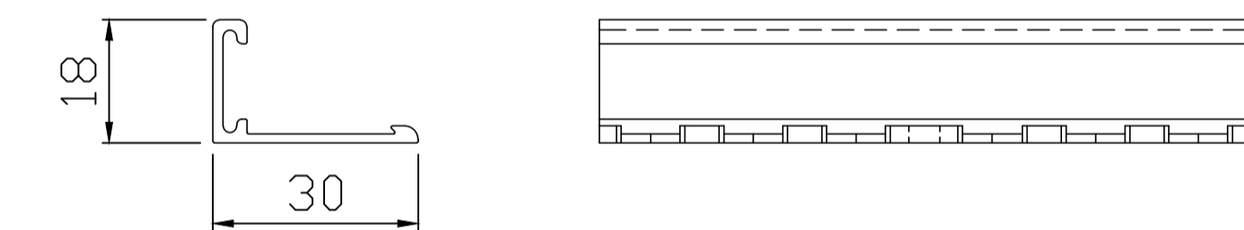
PROFILE DETAIL SCALE 1:1
